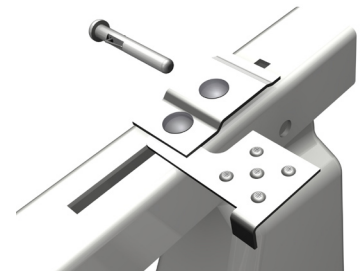
Tool-less Design
